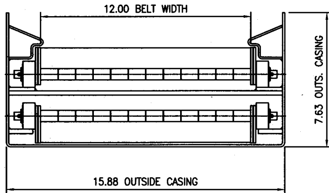
VIEW THRU CASING @ LOAD SECTION SCALE: (DOUBLE)
